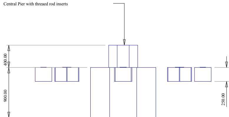
Central Pier with threaded rod inserts
